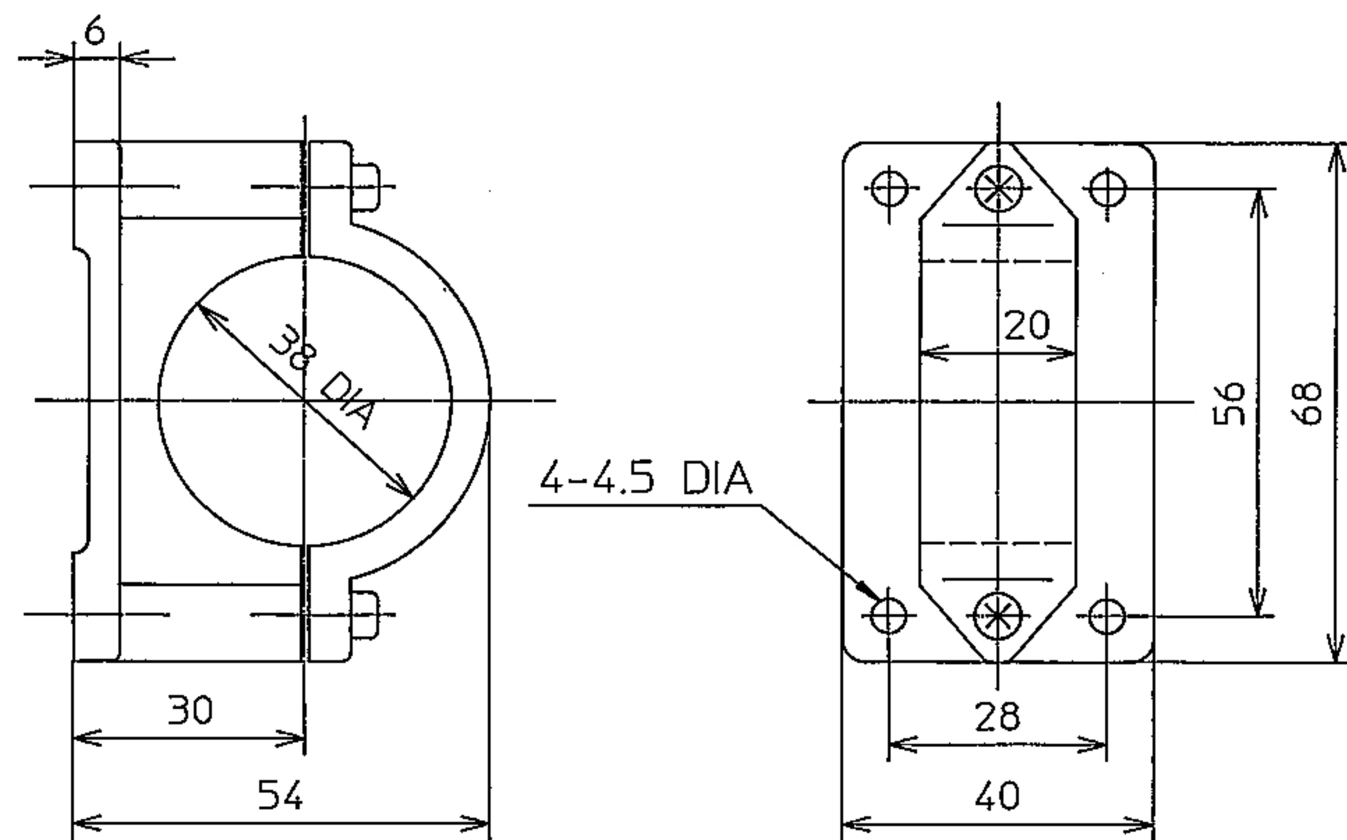
Mounting Block Type 2047
